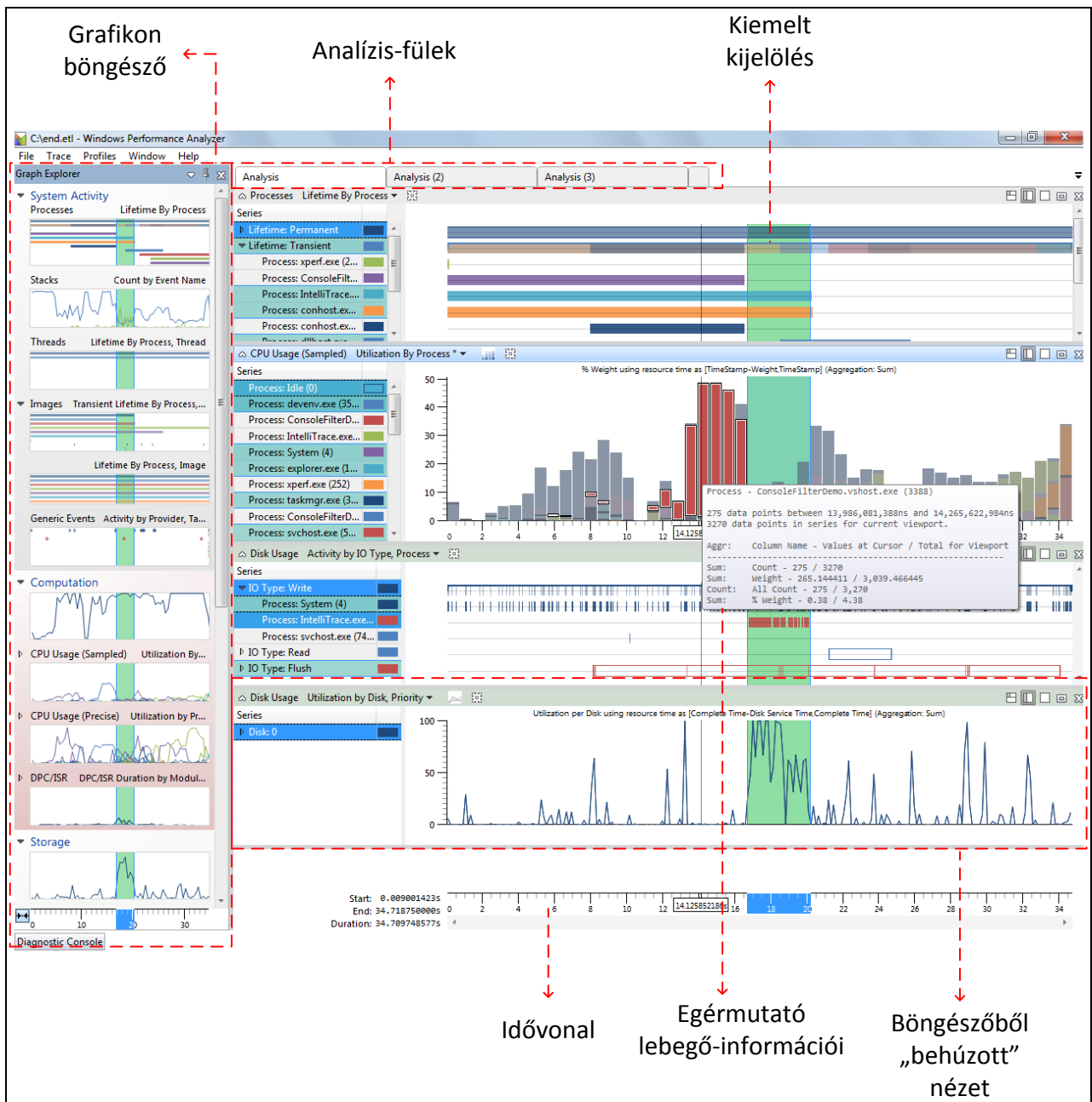
15. ábra Windows Performance Analyzer
