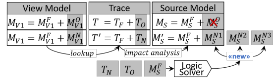
Figure 5. Overview of backward change propagation
