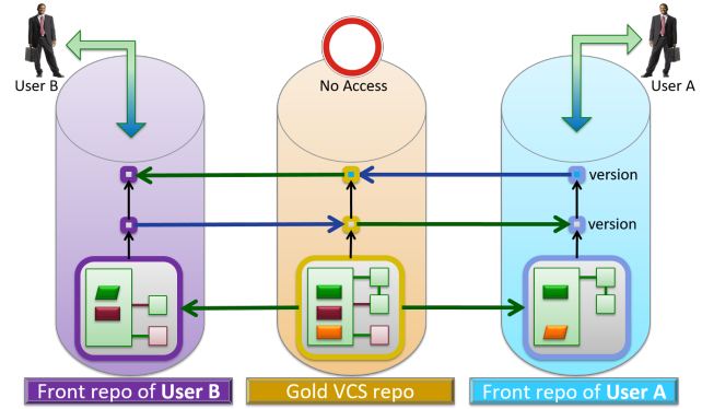
Figure 1. MONDO Offline Collaboration - Architecture
