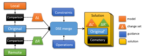
Figure 3. Architecture of DSE Merge
