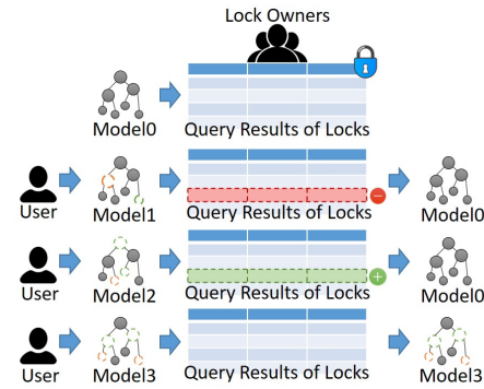
Figure 2. Behavior of Property-Based Locks
