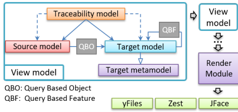
Figure 4. Overview of integration architecture
